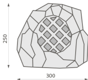
ROCCIA Dimensions: H250 x W300 x D230 mm Protection level: IP56
